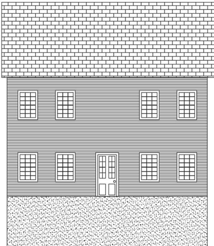
SOUTH ELEVATION
