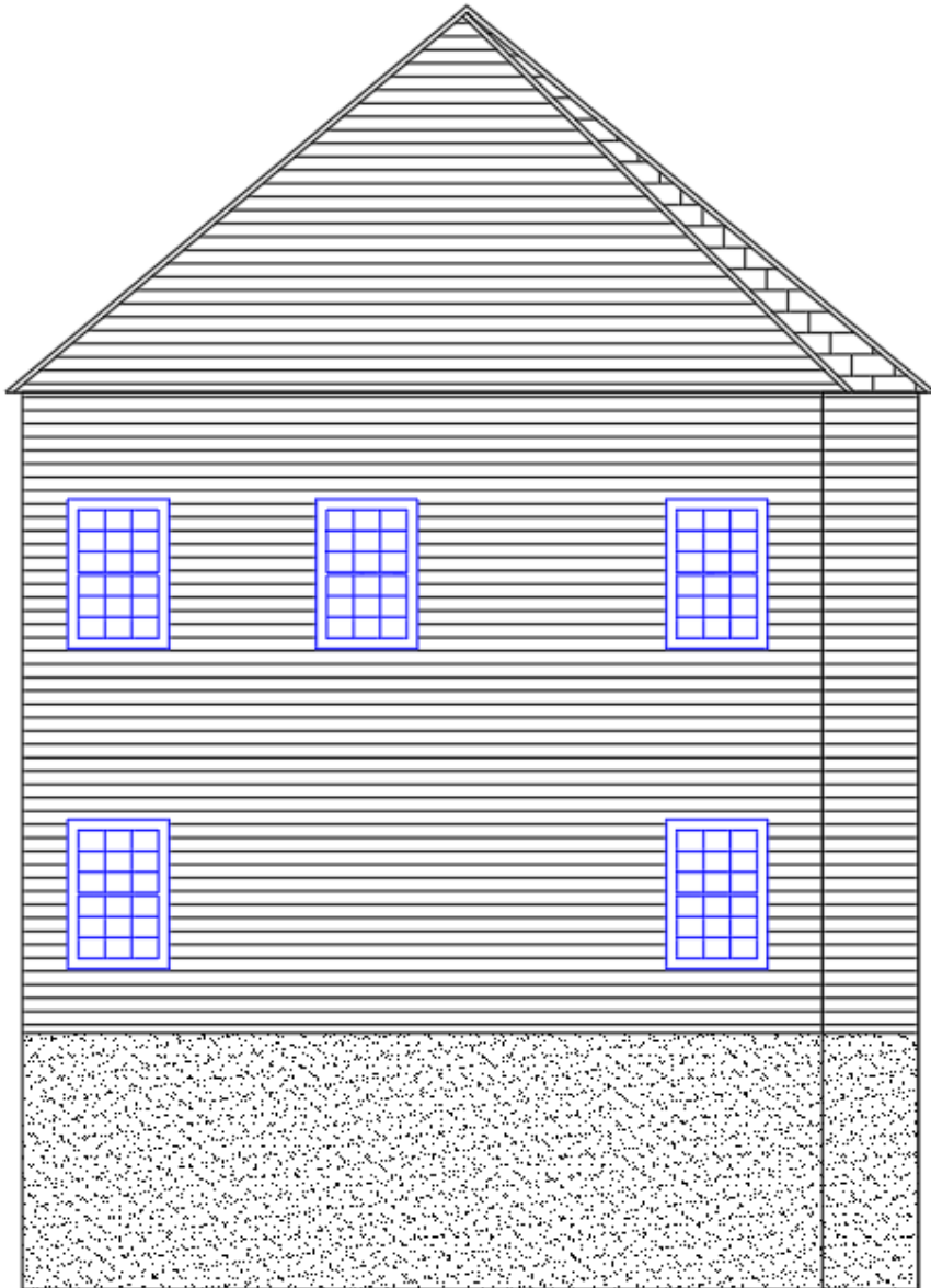
EAST ELEVATION
